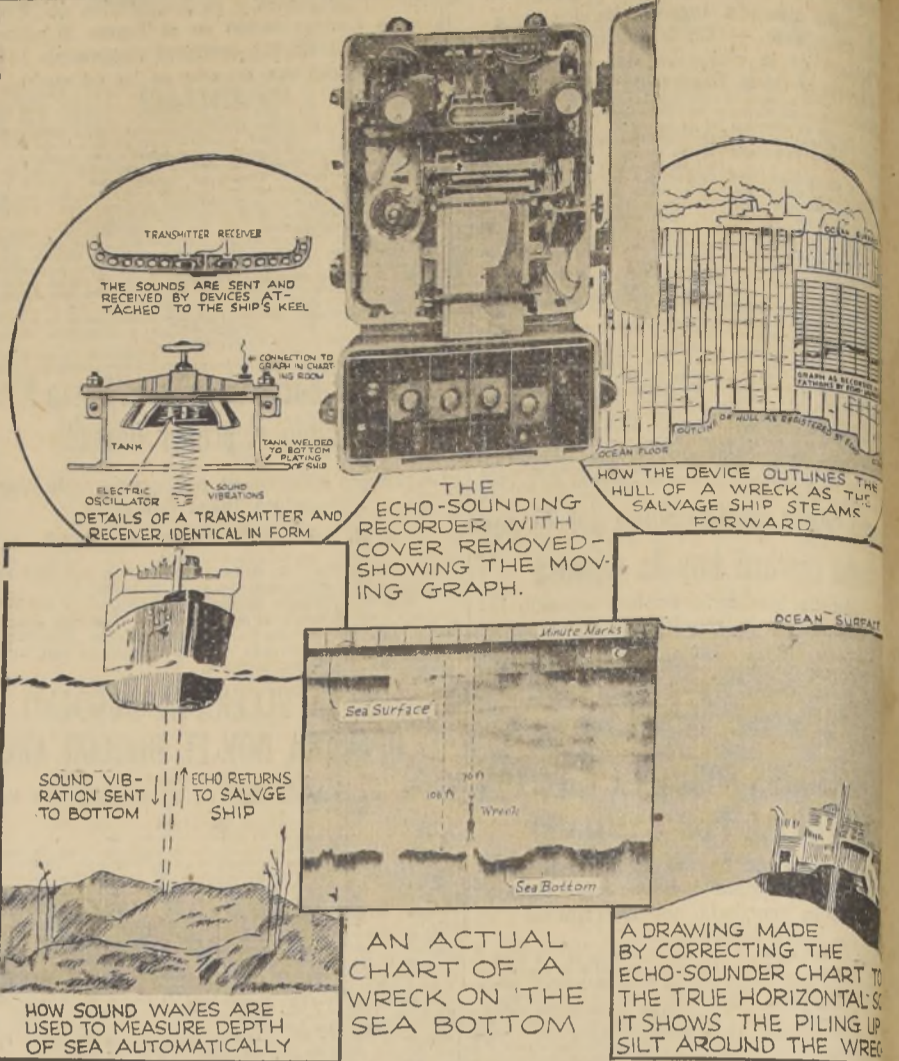
HOW SOUND WAVES ARE USED TO MEASURE DEPTH OF SEA AUTOMATICALLY
